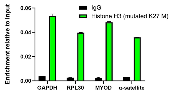
ChIP: Histone H3 (mutated K27 M)
