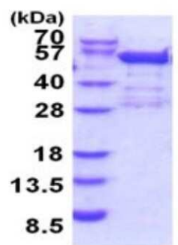
15% SDS-PAGE (3ug)
