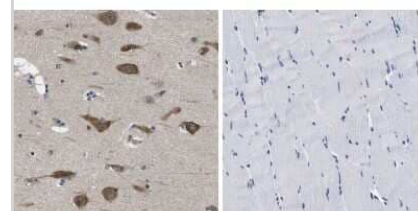
YARS in Cerebral cortex
