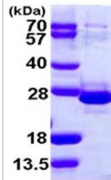
15% SDS-PAGE (3ug)
